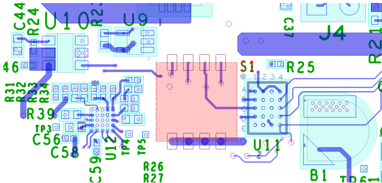
Figure 5 – SYSBOOT Switch Location
