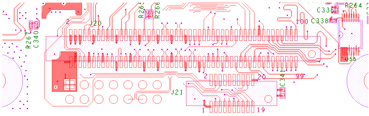
Figure 16 –Expansion Connectors - J20 and J21 (Bottom Side of PCB)
