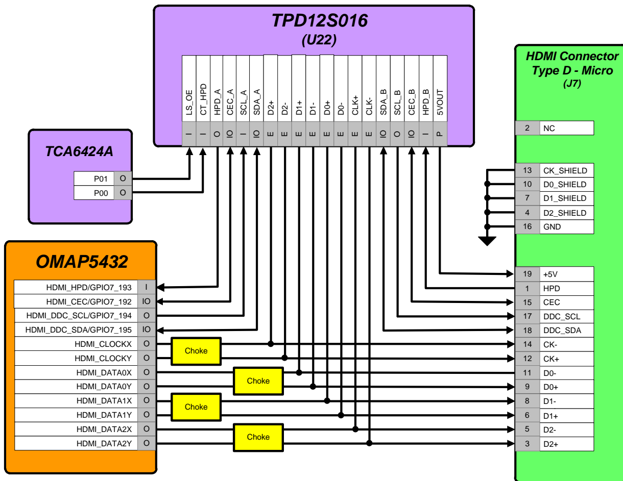
Figure 9 –HDMI Interface Block Diagram
