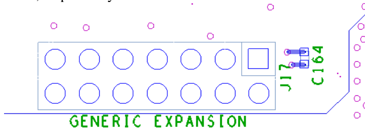
Figure 17 –Generic Expansion Connector – J17 (Top Side of PCB)
