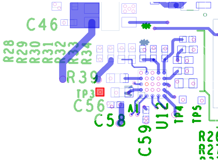
Figure 21 – USB Phy Ref Clock Probe Point (H_FREFCLK_1)
