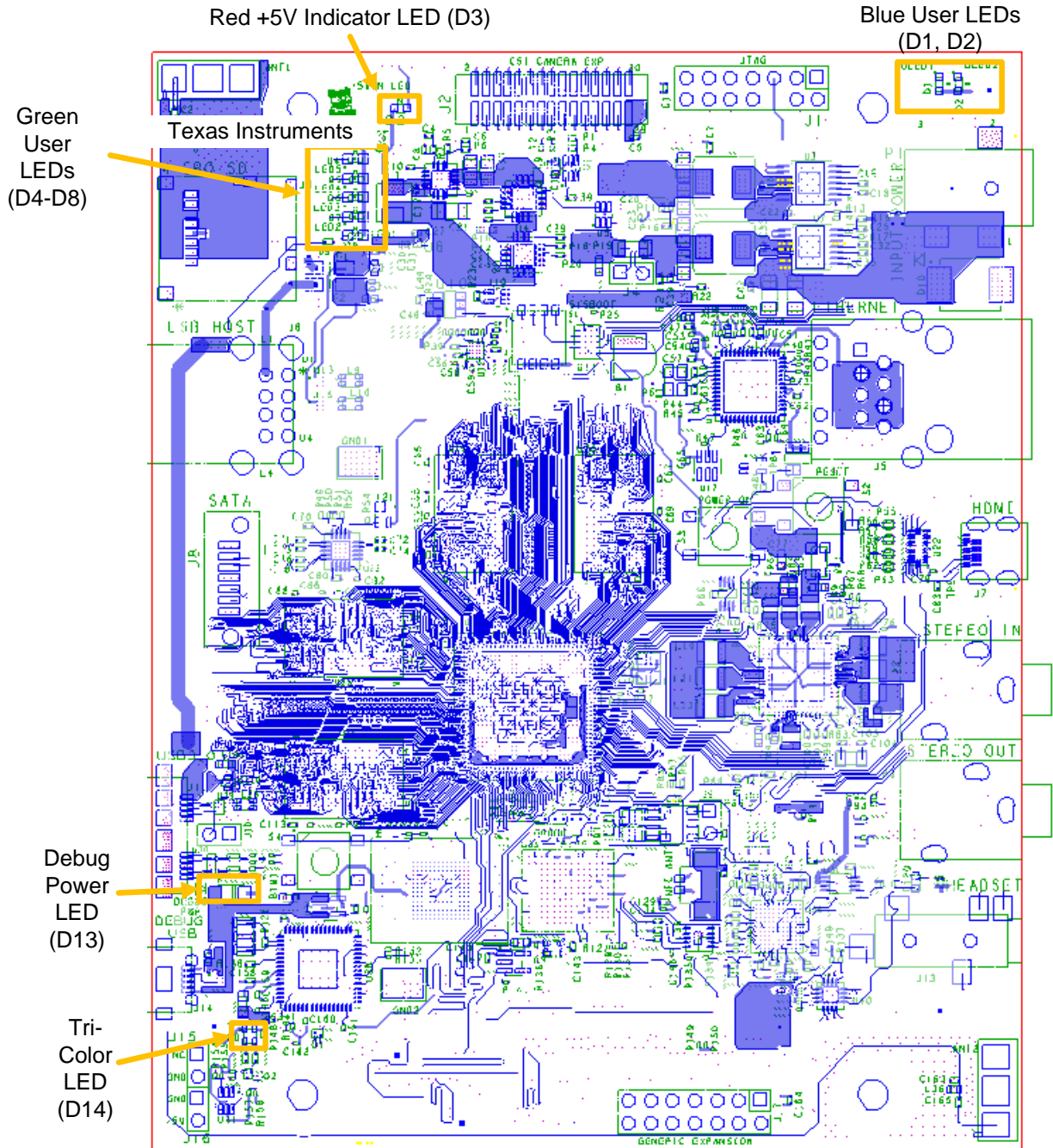
Figure 19 – LED Locations
