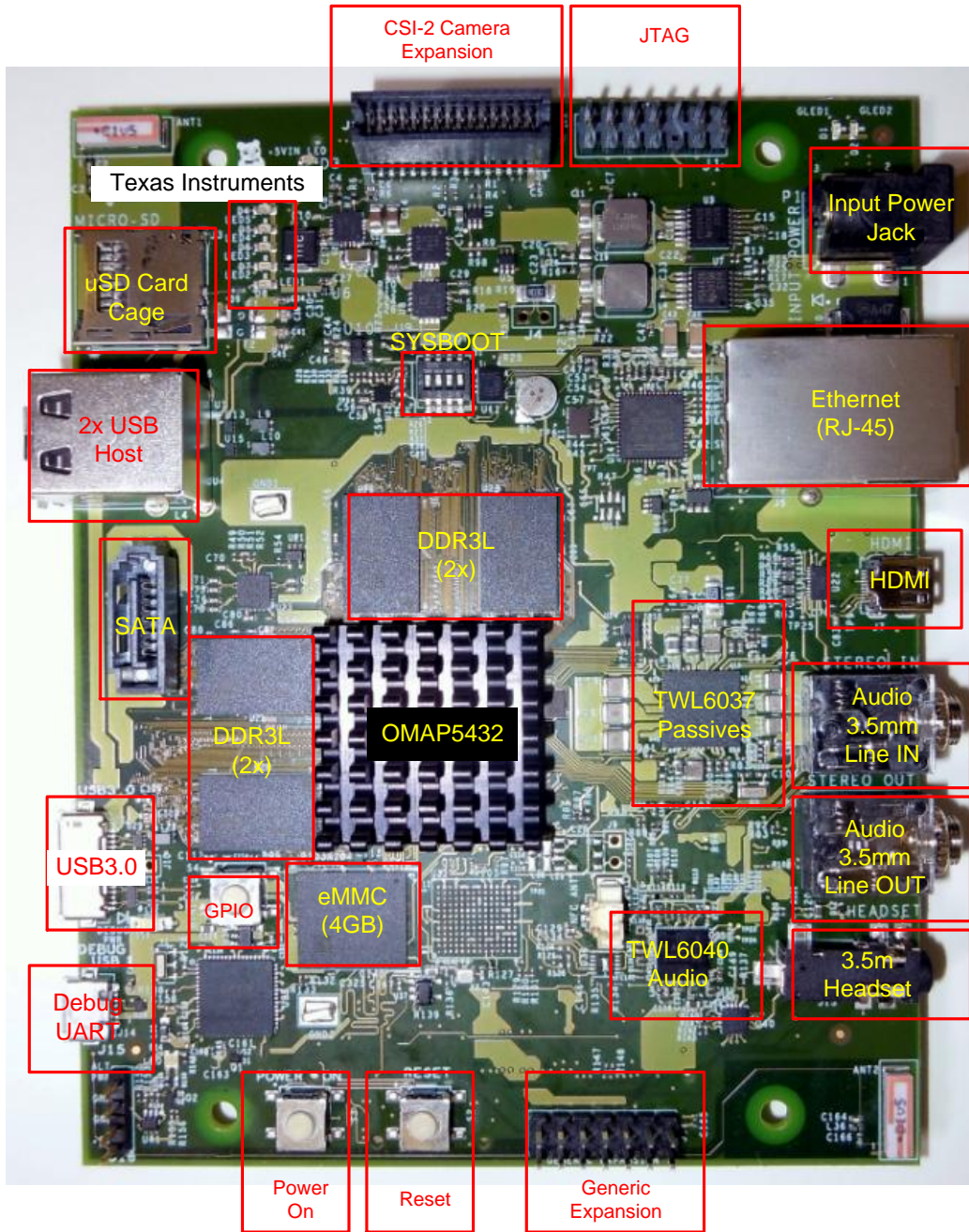
Figure 2 – OMAP5 EVM (Top View)
