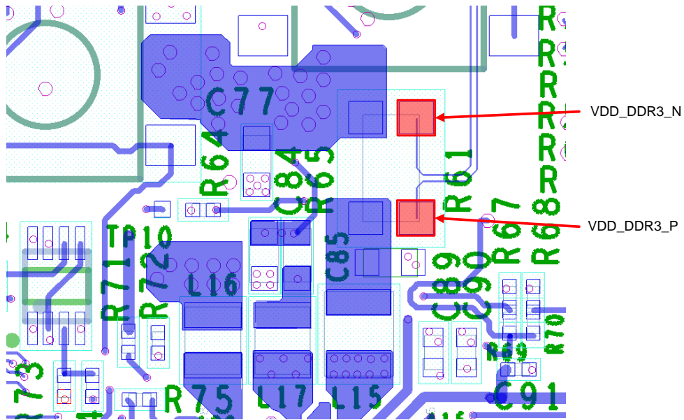
Figure 25 – DDR3 Current Measurement Probe Points (Top Side of PCB)
