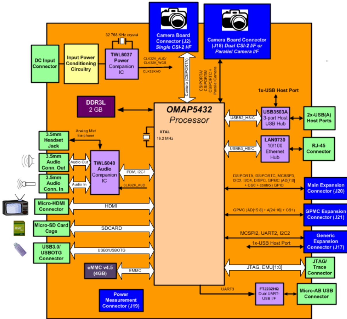
Figure 1 – OMAP5 EVM Architectural Block Diagram
