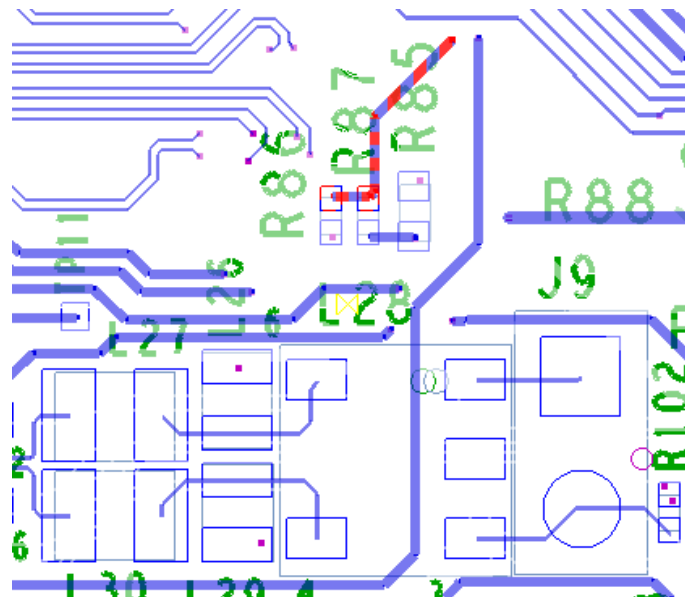
Figure 20 – High-Speed Audio Clock Probe Point (h_SYSCLK)
