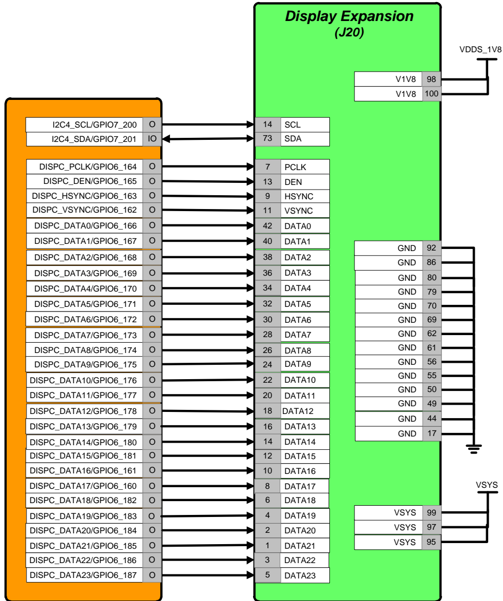
Figure 11 – Parallel Display on Expansion Connector (J20)
