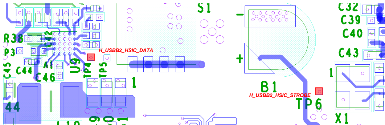
Figure 28 – USBB2 HSIC Interface Probe Points
