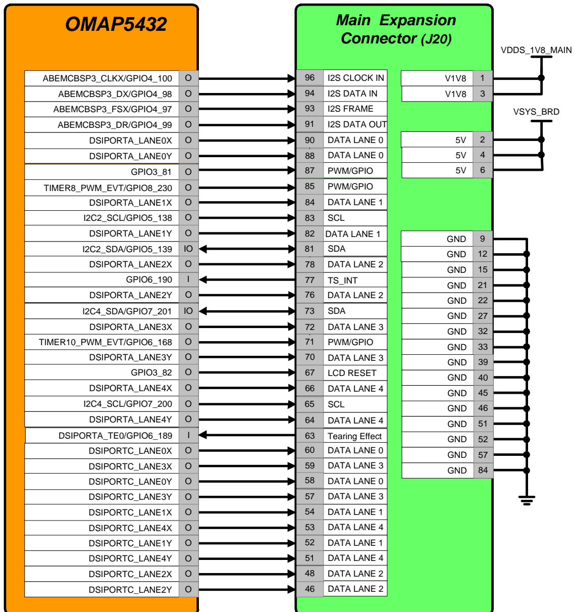
Figure 10 –DSI Display on Expansion Connector (J20)
