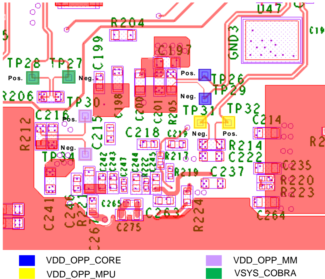
Figure 24 – OMAP5432 ES2.0 Current Measurement Probe Points (Back Side of PCB)
