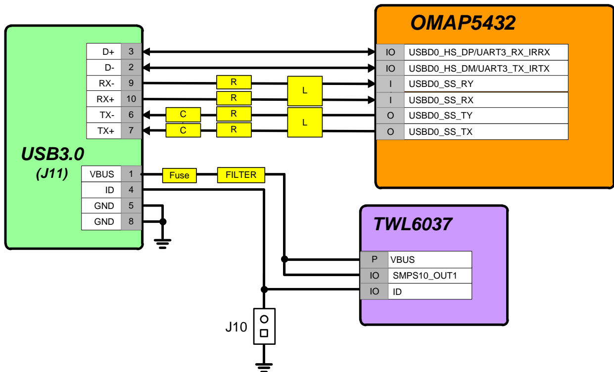
Figure 13 – USBOTG Interface Block Diagram
