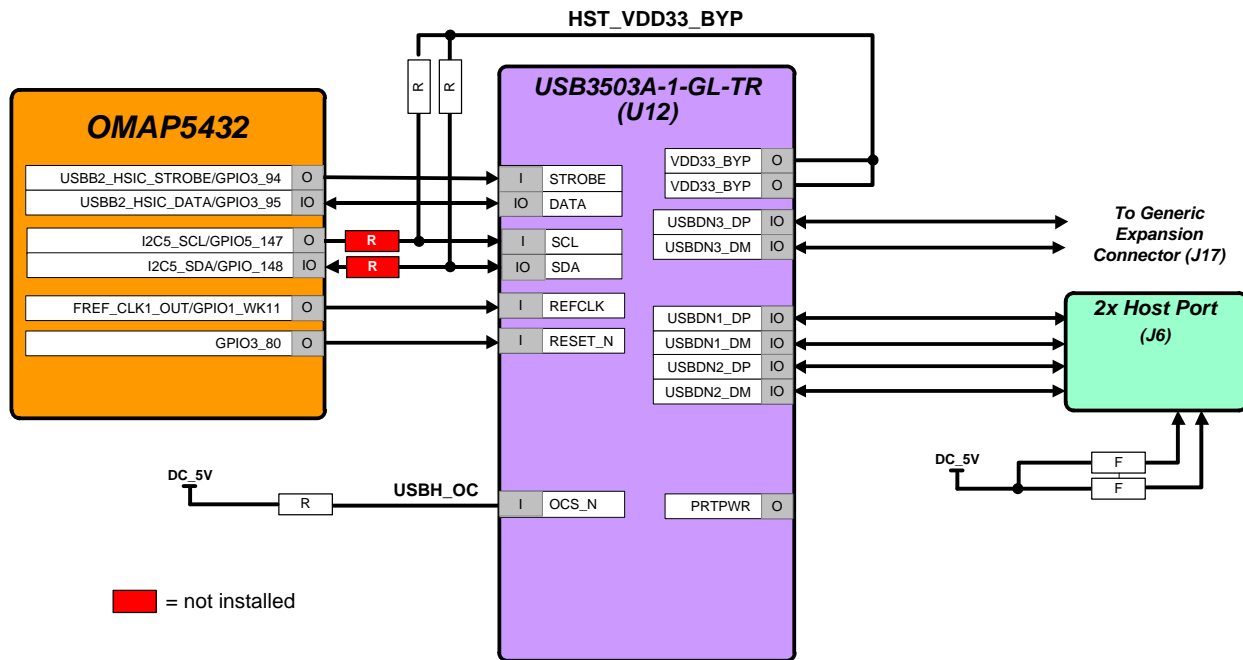
Figure 14 – USBB2 Interface Block Diagram
