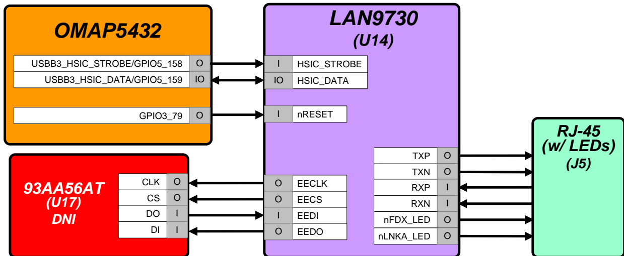
Figure 15 – USBB3 Interface Block Diagram
