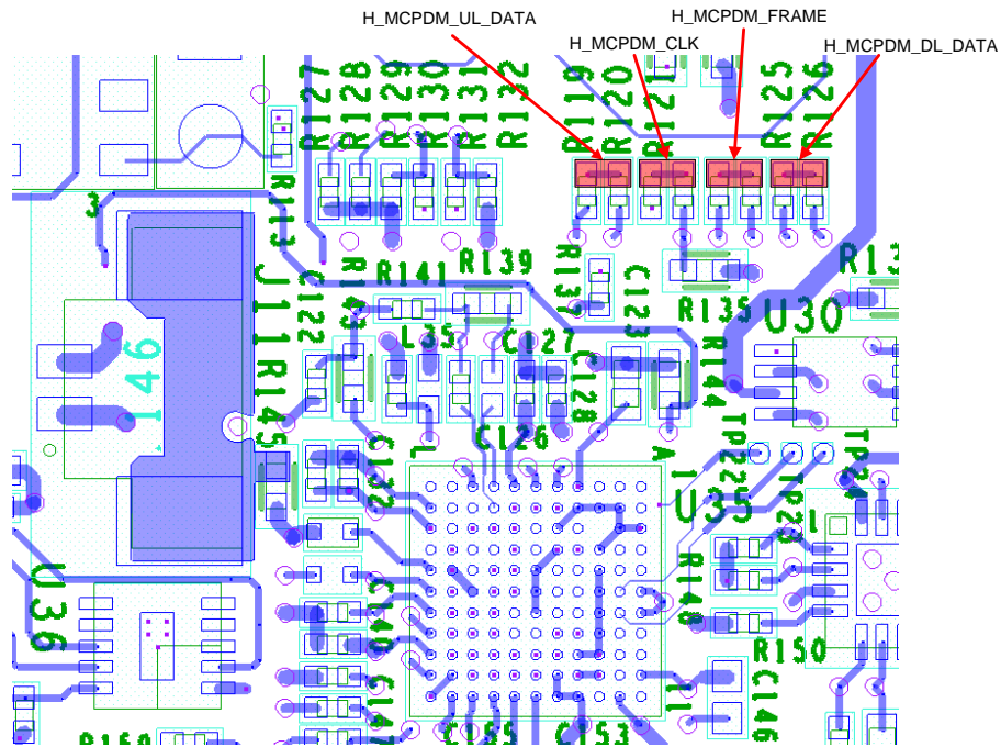
Figure 27 – TWL6040 PDM Interface Probe Points
