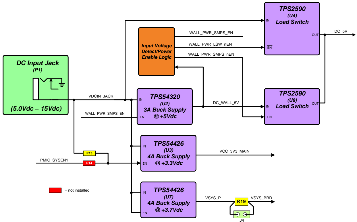
Figure 6 –Input Power Circuitry Block Diagram
