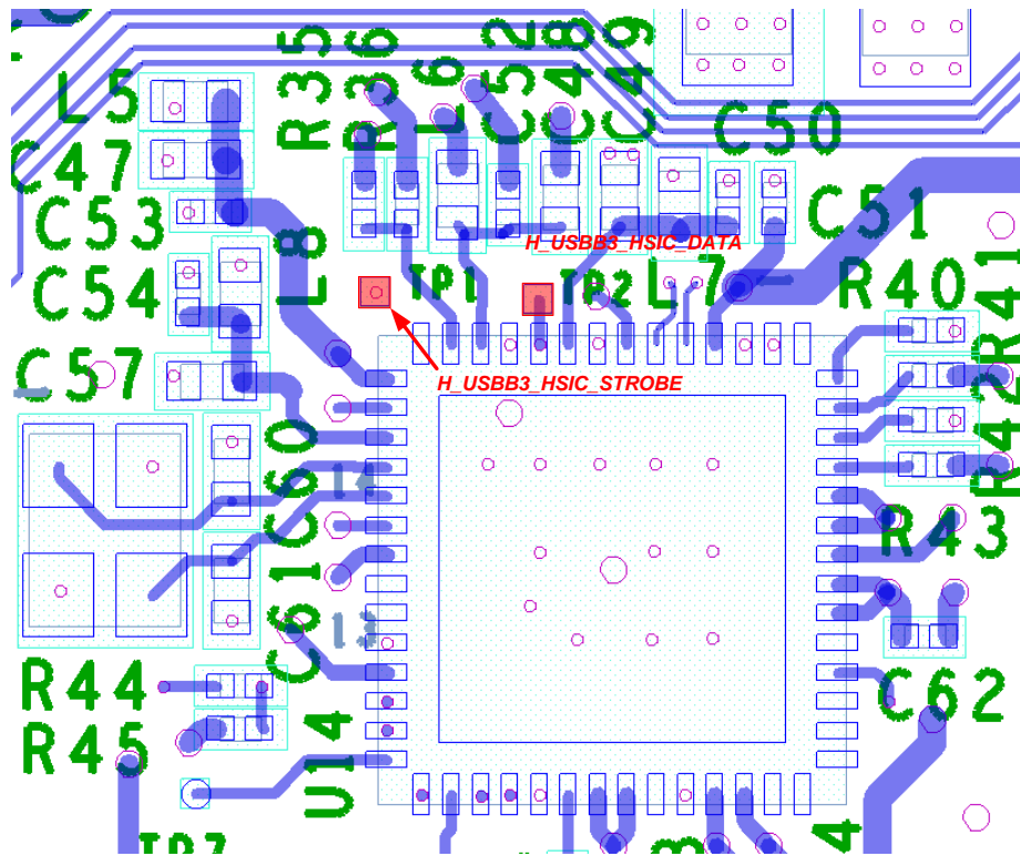
Figure 29 – USB3 HSIC Interface Probe Points
