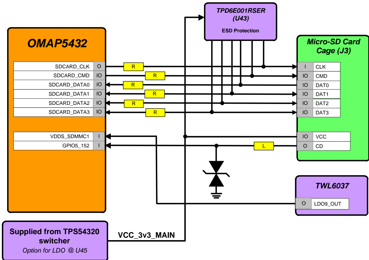
Figure 8 –SDMMC1 Card Cage Block Diagram
