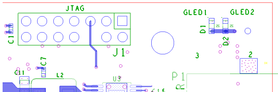
Figure 18 – 14-pin JTAG Connector (J1)
